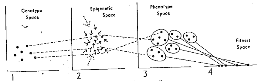
FIG. 2.—Waddington's epigenetic space
