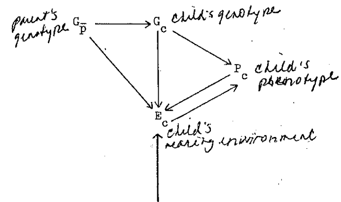
FIG. 1.—A model of behavioral development
