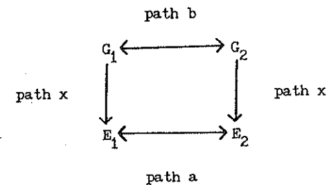
FIG. 3.—A model of environmental similarity based on genetic resemblance.
