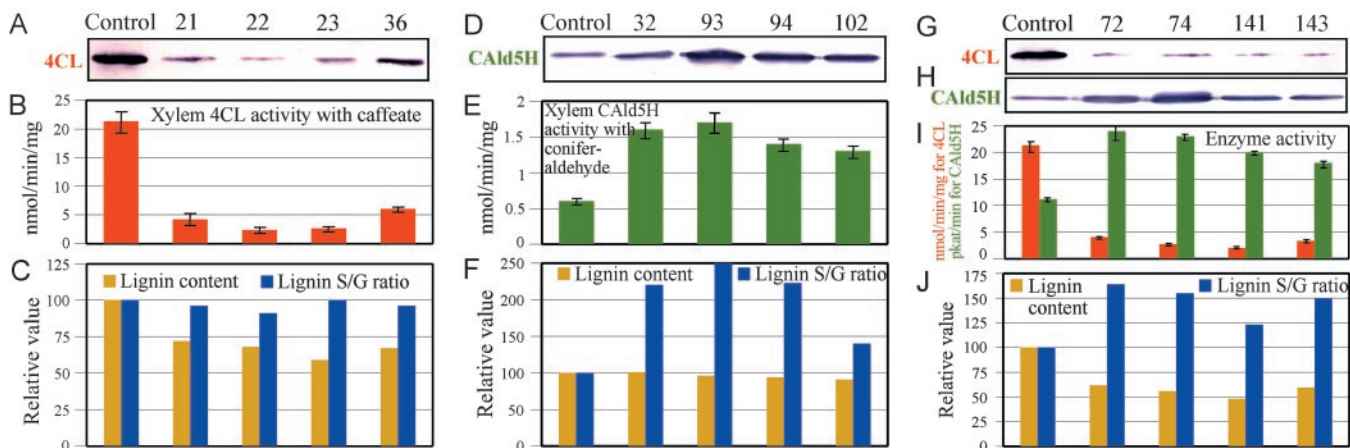
Fig. 3. The effects of down-regulation of 4CL and up-regulation of Cald5H on 4CL and CAld5H enzyme activities and lignin accumulation and S/G ratio. (A, D, G, and H) Protein gel-blot (10 μg of protein extracts per lane) analysis of xylem 4CL and CAld5H protein levels by using anti-4CL (A and G) and anti-CAld5H (D and H) antibody probes, respectively. (B, E, and I) 4CL and CAld5H enzyme activities in stem developing xylem tissue. Crude protein (20–40 μg) was assayed for 4CL (B and I) and CAld5H (E and I) activities with caffeate and conifer-aldehyde, respectively, by using HPLC/MS. Error bars represent standard deviation values of three replicates. (C, F, and J) The levels of lignin reduction and lignin S/G ratio increase in stem wood of transgenic lines as compared with the control.
